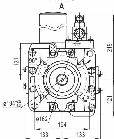
PVH2.75
