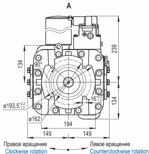
PVH2.90, PVH2.112
