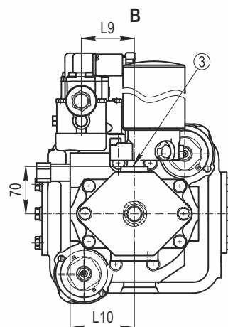
PVH2.90, PVH2.112
