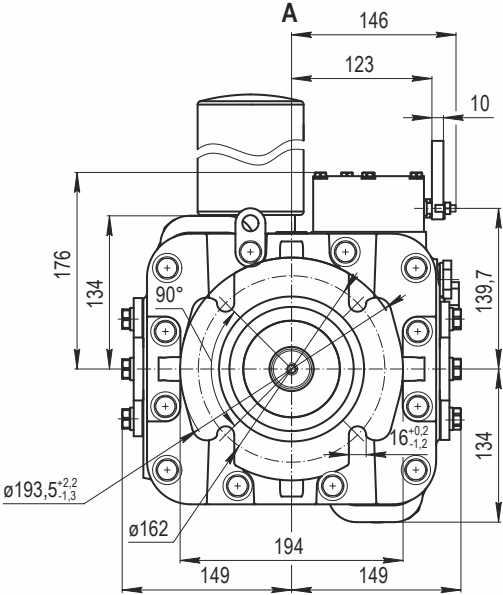
PVH2.90, PVH2.112
