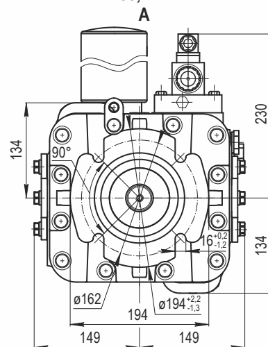
PVH2.90, PVH2.112
