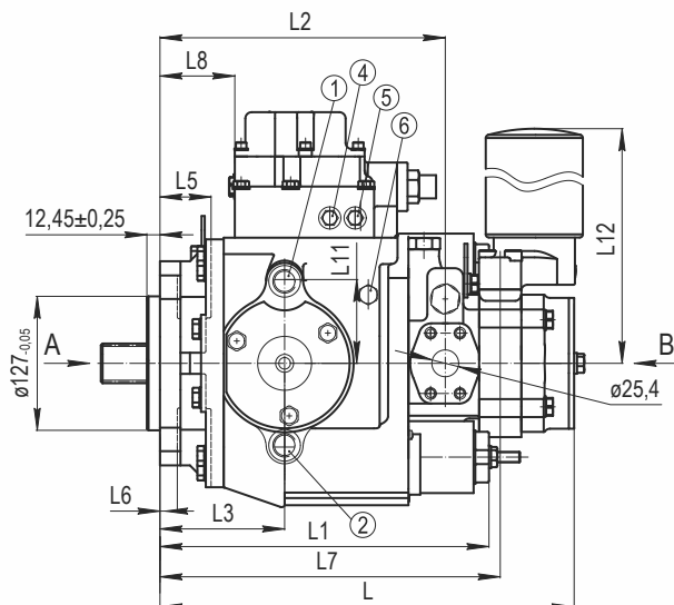
PVH2.75
