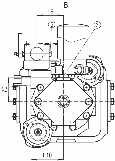
PVH2.90, PVH2.112
