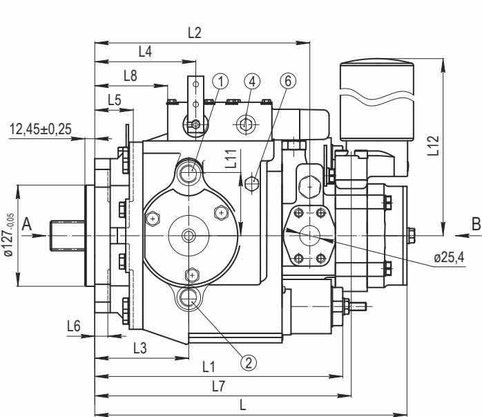
PVH2.75
