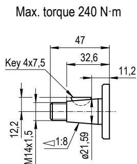
G4 EUROPEAN TAPERED 1:8
