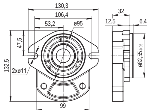
31 SAE A 2 BOLTS
