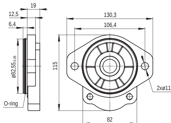
32 SAE A 2 BOLTS (WITH O-RING)
