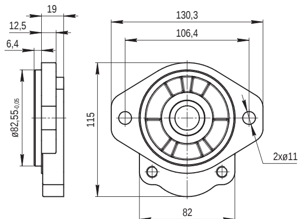
31 SAE A 2 BOLTS
